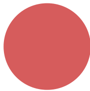
AMBROSIAQSR AGGRESSIVE
