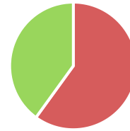
AMBROSIAQSR MODERATE
