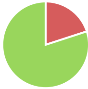
AMBROSIAQSR CONSERVATIVE
